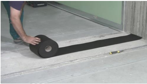
Lay the under wall strip in the dry floor.
